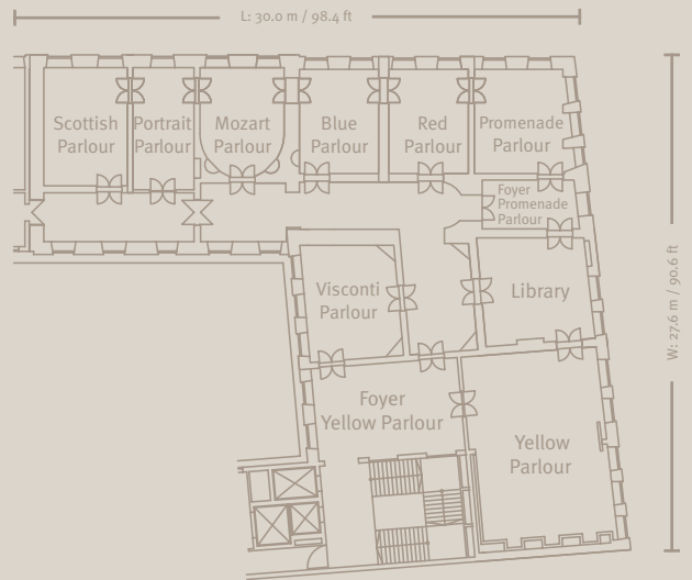
Palais Montgelas, 1st floor: 448.6 sqm / 4,828.7 sqft
